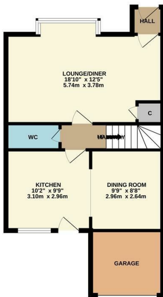
GROUND FLOOR 536 sq.ft. (49.8 sq.m.) approx.
